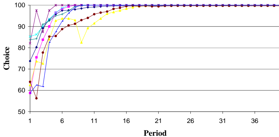
Figure 2: Treatment 2 - group averages ( p = 2/3 ; d = 50 )
